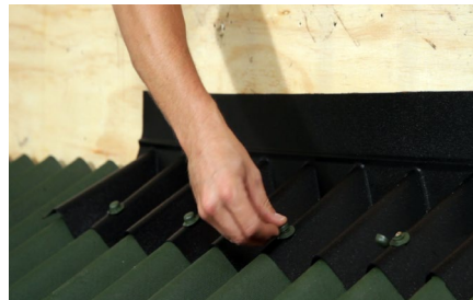
Onduline apron fixing Use Onduline pre-formed apron flashing piece to seal end wall abutments. Lay the upstand against the wall and fix the front apron at each corrugation.
